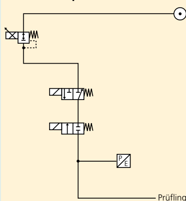
Functional diagram Relative-pressure method
