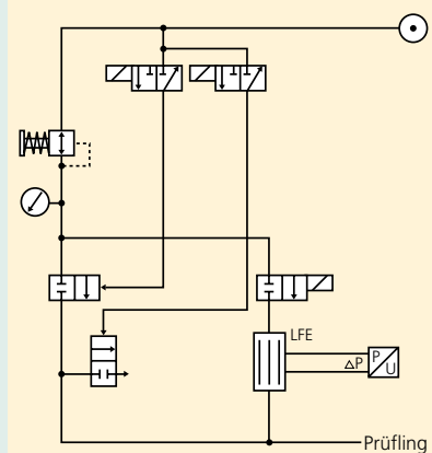
Functional diagram Flow method (volume flow)
