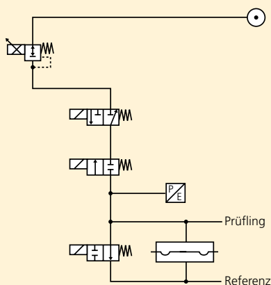
Functional diagram Differential-pressure method
